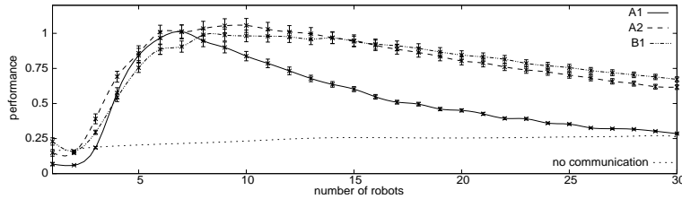
Fig. 5. Performance of A1 , A2 , and B1 individuals. For each group size several simulation runs ( N = 25 ) were performed, each lasting 18,000 time steps. Performance is the mean number of finding a food patch in 600 time steps for a single robot (mean of all robots in a group is taken). The mean performance of A1 , A2 , and B1 individuals where the communication system was deactivated is drawn as a reference (dotted line).
